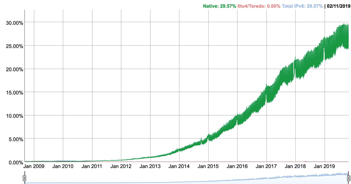
IPv6 Adoption
